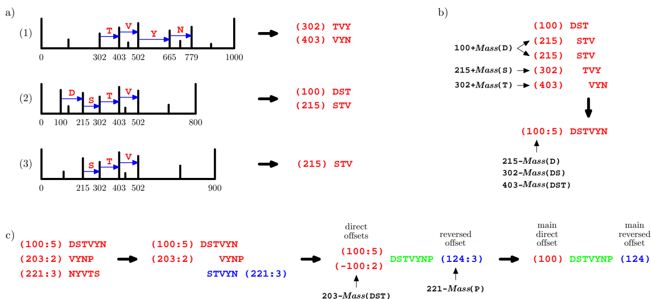
Fig. 1. Overview of the entire method for aggregated strings generation. a) Extraction of 3-tags from the input set of deconvoluted MS/MS spectra. b) Assembly of a de novo string from five 3-tags consistent with each other in terms of both amino acid sequences and offsets. The resulting de novo string “DSTVYN” is assigned the mass offset of 100 with multiplicity 5. c) Formation of an aggregated string from three de novo strings endowed with offsets. The resulting aggregated string “DSTVYNP” has the main direct and reversed offset of 100 and 124, respectively, which leads to the precursor mass estimate PM_{\text{DSTVYNP}} = 100 + \text{Mass}(\text{DSTVYNP}) + 124 = 1000 .
