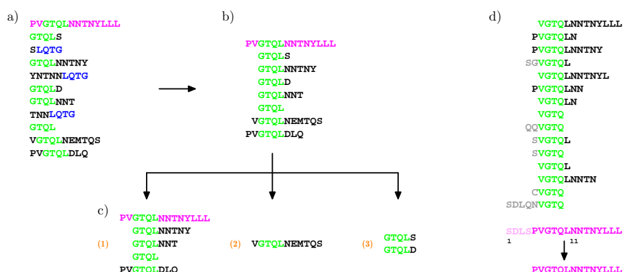
Fig. 3. a)-c) Processing the alemtuzumab dataset: handling the 4-mer “GTQL” with the score 8. a) The set of active strings containing “GTQL” or “LQTG”. b) The aligned strings (duplications due to string reversal are not shown). c) Clusterization: the string “VGTQLNEMTQS” did not match well the main string “PVGTQLNNTNYLLL”, and gave rise to the second cluster; each of the strings “GTQLS” and “GTQLD” produced one mismatch when being aligned against “PVGTQLNNTNYLLL” or “VGTQLNEMTQS”, and thus, both were placed in the third cluster. d) The aggregated string with the amino acid sequence “PVGTQLNNTNYLLL” (depicted in magenta) was obtained at time of processing the 4-mer “VGTQ” with the score 25. The first four amino acids of its underlying consensus string “SDLSPVGTQLNNTNYLLL” were eliminated by the validation procedure. Incorrect candidate amino acids in the aligned strings are marked gray (the amino acid scores are not shown). A 4-mer being processed and its reversed copy are highlighted green and blue, respectively.
