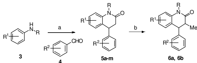
Scheme 1. (a) Meldrum's acid, EtOH, 85°C, 16 h (55-78%); (b) BuLi, THF, 0°C then MeI (48%).
