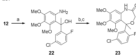
Scheme 5. (a) MeMgBr, THF, 0°C (67%); (b) BrCH 2 C(O)Cl, Et 2 O, Et 3 N, 0°C to RT; (c) NaH, THF, RT then reflux (54% over 2-steps).
