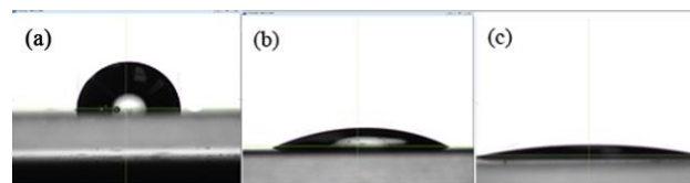
Figure 5. Hydrophilicity test on differently treated PS film. Only PS film in the device has direct surface contact with reactant, thus it is specially treated to acquire different surface property. (a) without treatment, contact angle= 92^\circ (b) PS film after oxygen plasma treatment, contact angle= 25^\circ (c) PS film after hydrophilic coating, contact angle= 17^\circ
