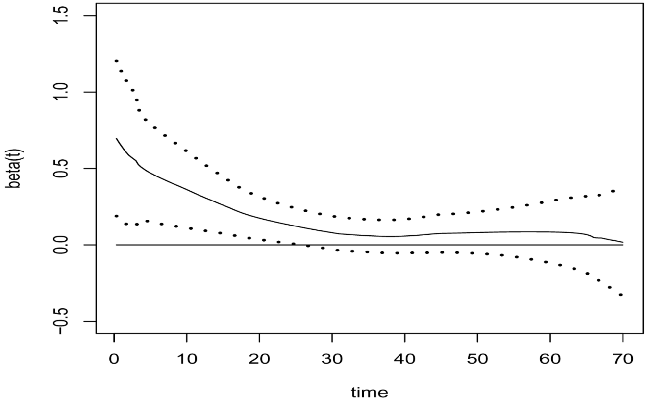
Figure 5.2. The kernel estimator and 95% confidence interval of the varying coefficient function of LNBPD for the western Kenya parasitemia data, bandwidth h = 25
