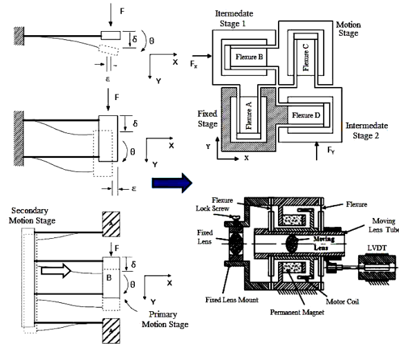
Figure 2. Mechanisms developed using planar flexible joints
