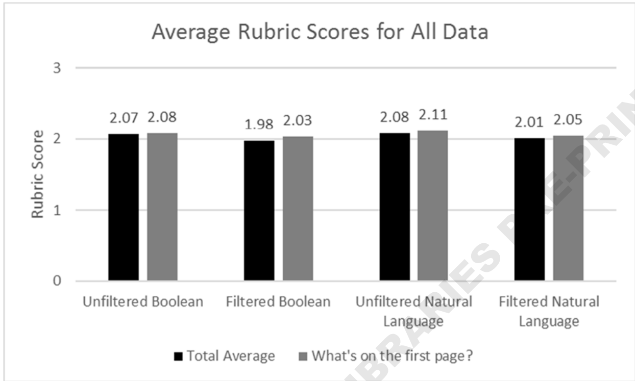
Chart 1 – Average Rubric Scores for All Data
