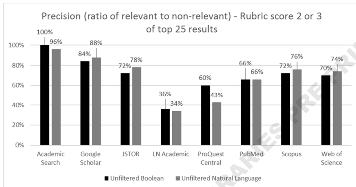
Chart 8 – Precision (ratio of relevant to non-relevant) – A Rubric Score of 2 or 3 of the top 25 results
