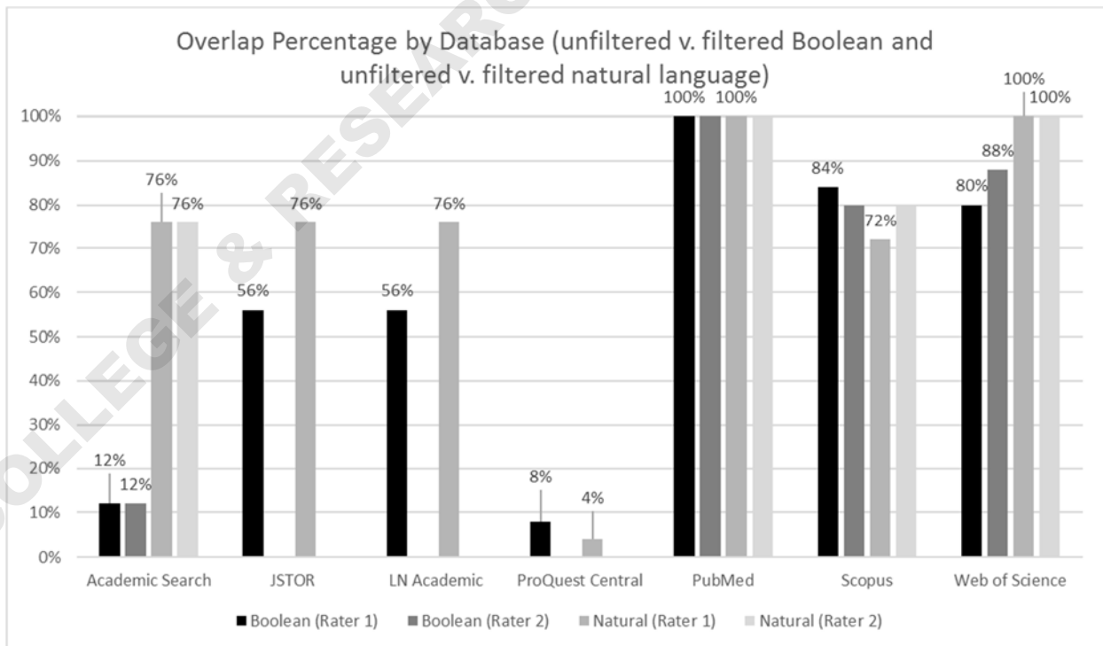
Chart 7 – Overlap Percentage by Database (unfiltered/filtered Boolean and unfiltered/filtered natural language)
