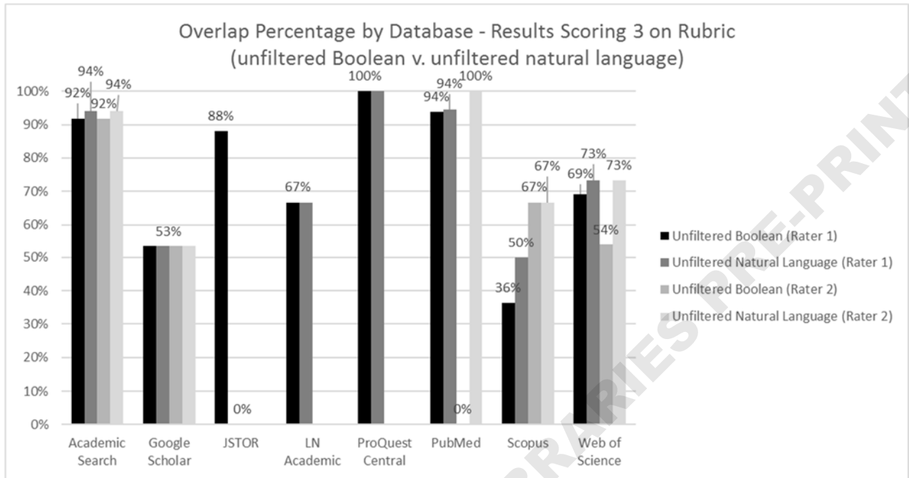
Chart 6 – Overlap Percentage by Database – Results Scoring Three on the Rubric (unfiltered Boolean v. unfiltered natural language)
