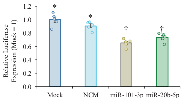
Fig. 3 MiR-20b target conservation on APP 3'-UTR and site confirmation. A The hsa-miR-20b sequence was used to probe the APP 3'-UTR sequence with the STarMir utility. [57] A single putative site was predicted, with 100% homology to the 8-base seed sequence. Additional miRNA species previously confirmed to regulate APP translation are also shown [39–42]. B Multiple sequence alignment of homologous regions from 12 additional mammalian species. Seed sequence (outlined) was conserved across multiple genera and families. Homology was compared between each animal target sequence and hsa-miR-20b-5p sequence and vs. the human 3'-UTR target sequence. All sequences maintained at least 63% homology to complete miR-20b-5p sequence and at least 91.3% homology to the human target sequence. C APP 3'-UTR-coupled-reporter activity. Reporter clone with full APP 3'-UTR sequence was co-transfected with NCM and miR-101-3p and miR-20b mimics. miR-20b significantly ( p \leq 0.05 ) reduced levels of luciferase reporter expression. Symbols indicate estimated marginal means categories. Samples sharing a symbol did not significantly differ from each other. Error bars represent standard errors of means (SEM).
